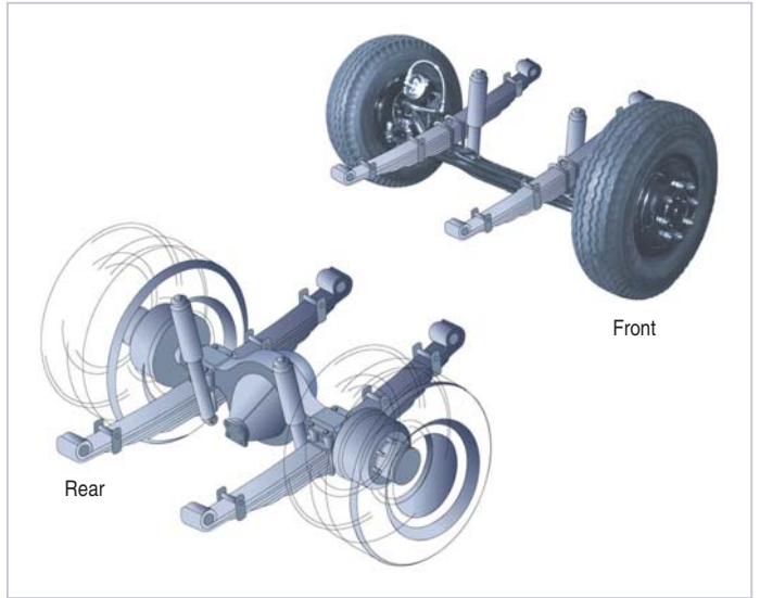
Leaf suspension
