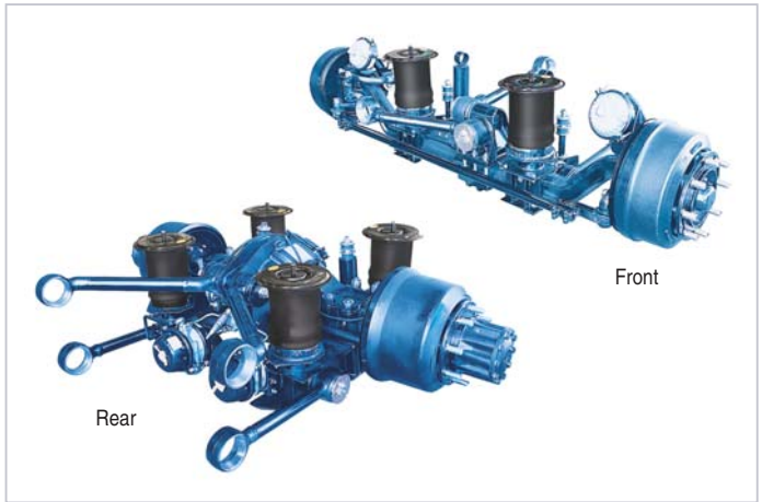
FRT / RR air suspension
